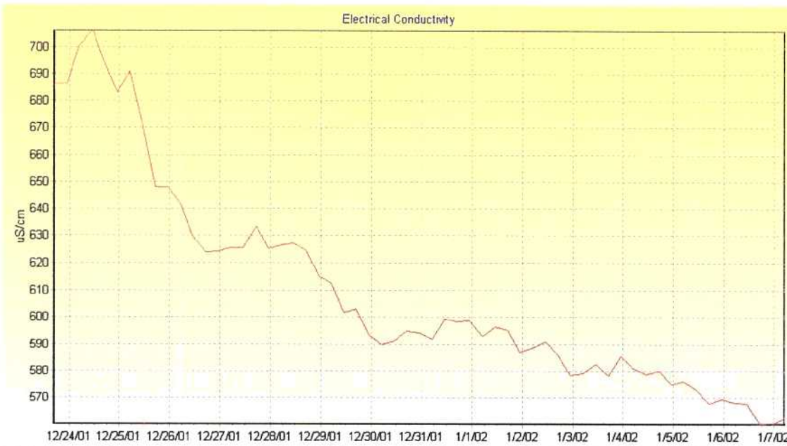
Figure 26. Detailed electrical conductivity data obtained by double-clicking on EC image on real-time SJR DO project website for the West Stanislaus monitoring station.
