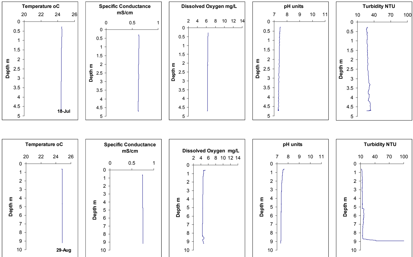
Fig. II-3a. Vertical profiles of water quality variables near Turner Cut
