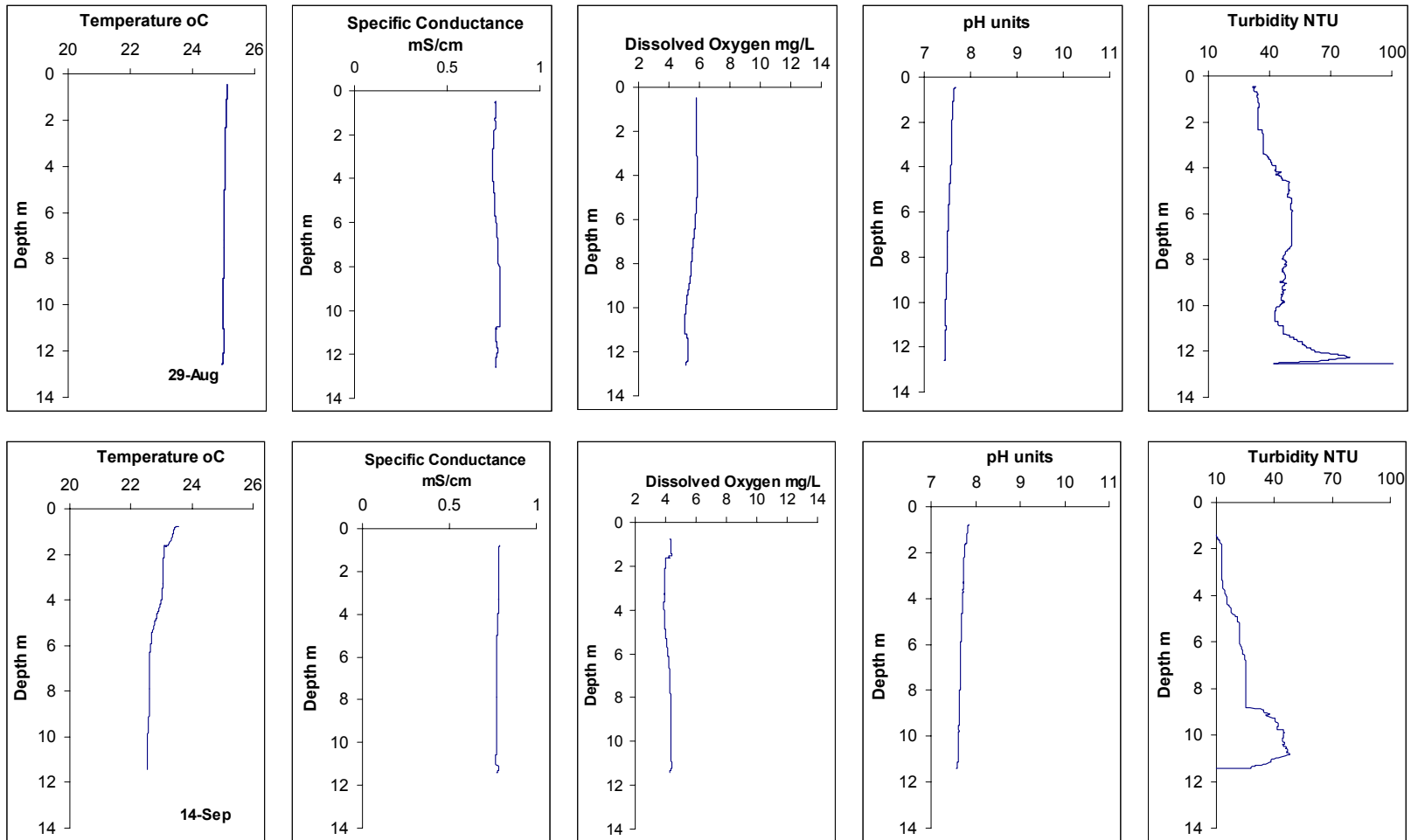
Fig. II-3c. Vertical Profiles of water quality variable near Light 48.
