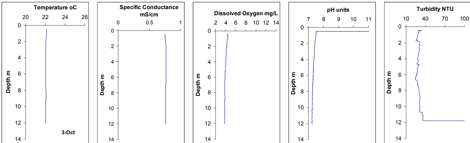
Fig. II-3c. Vertical Profiles of water quality variable near Light 48.
