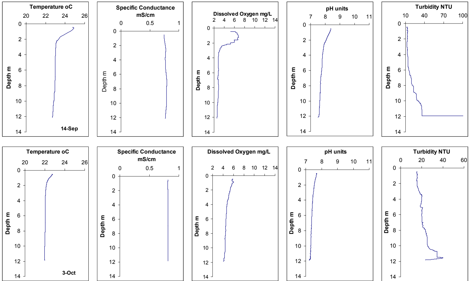
Fig. II-3b. Vertical Profiles of water quality variable near Rough and Ready.
