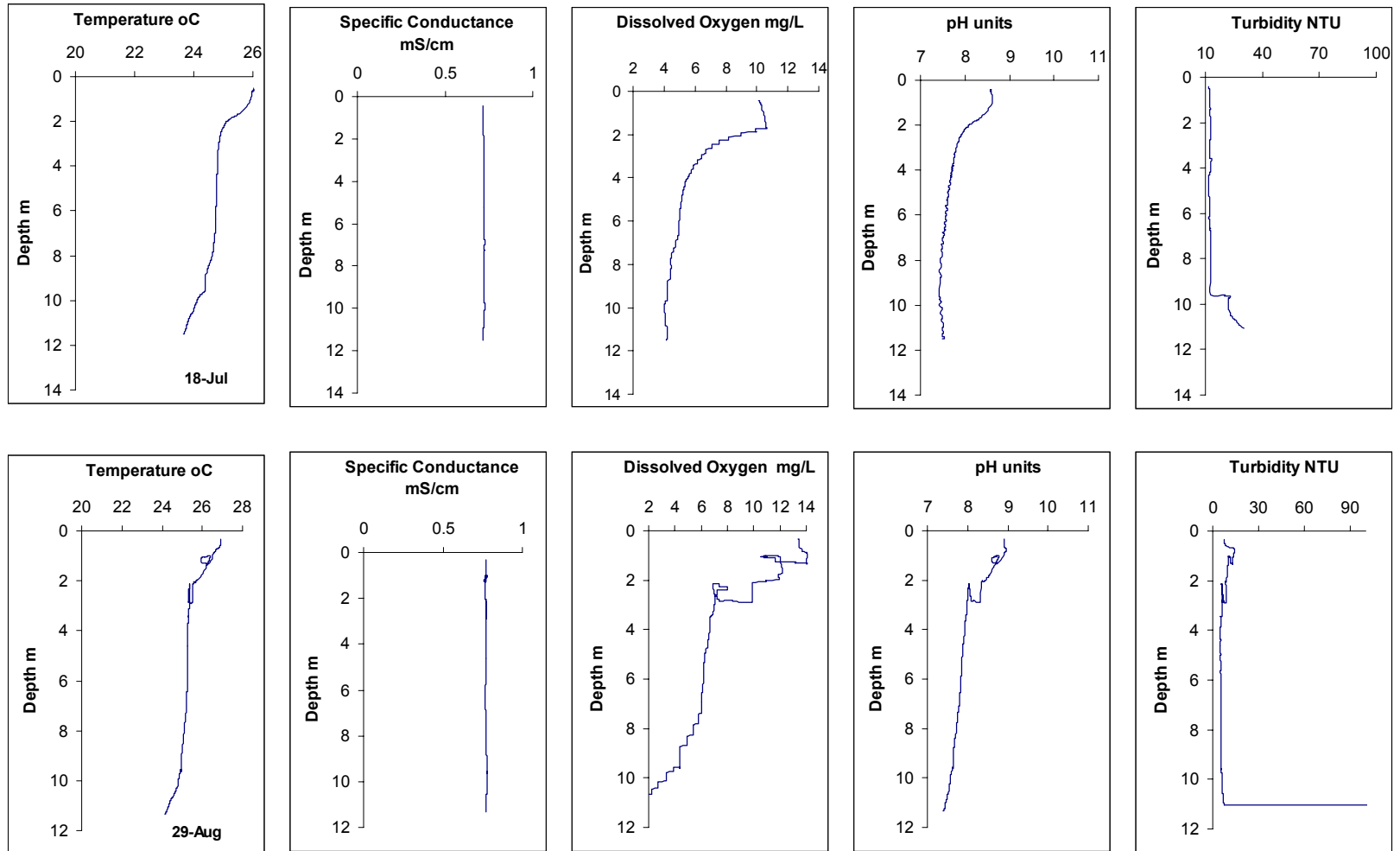
Fig. II-3d. Vertical Profiles of water quality variables near Turning Basin.
