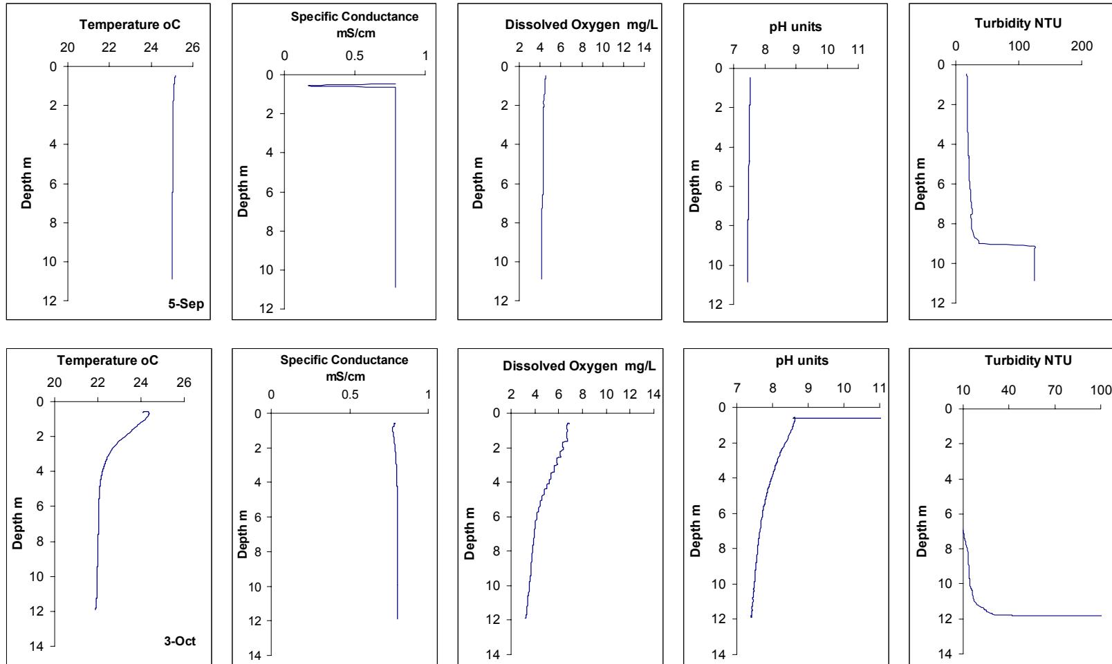
Fig. II-3d. Vertical Profiles of water quality variable near Turning Basin.
