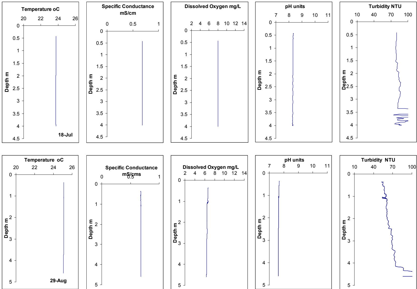
Fig. II-3e. Vertical profiles of water quality variables near Channel Point.
